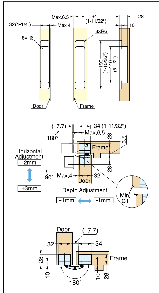
Bore Dimensions
